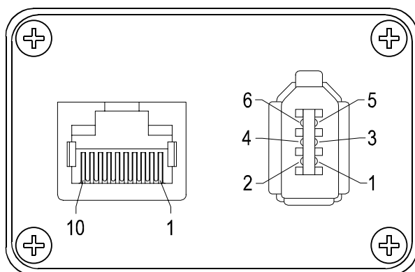
Figure 2-2: A630f Pin Numbering
