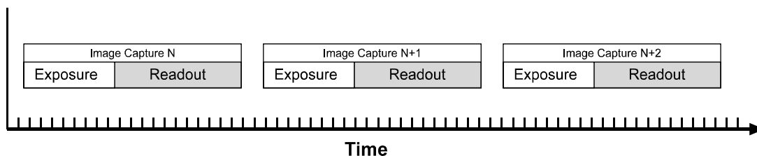
Figure 3-6: Non-overlapped Exposure
