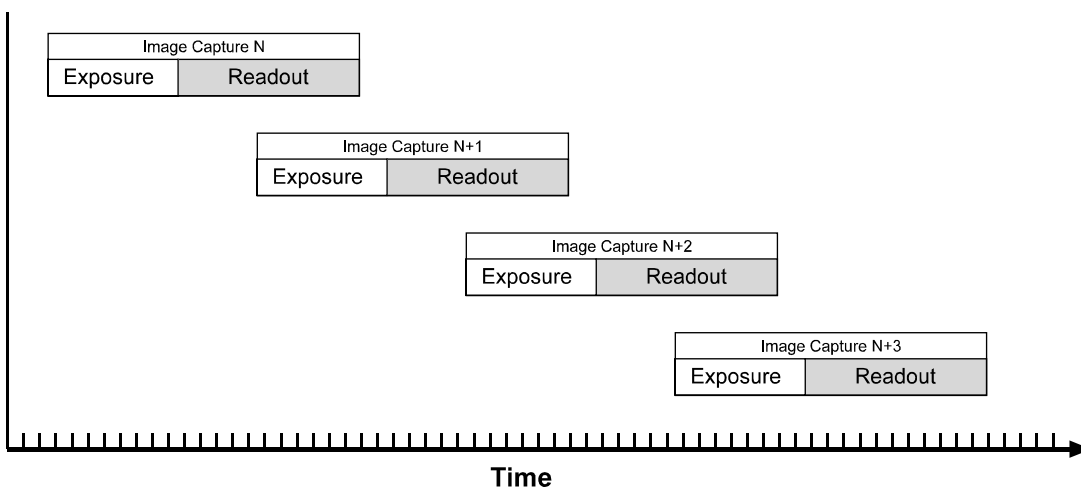
Figure 3-7: Overlapped Exposure
