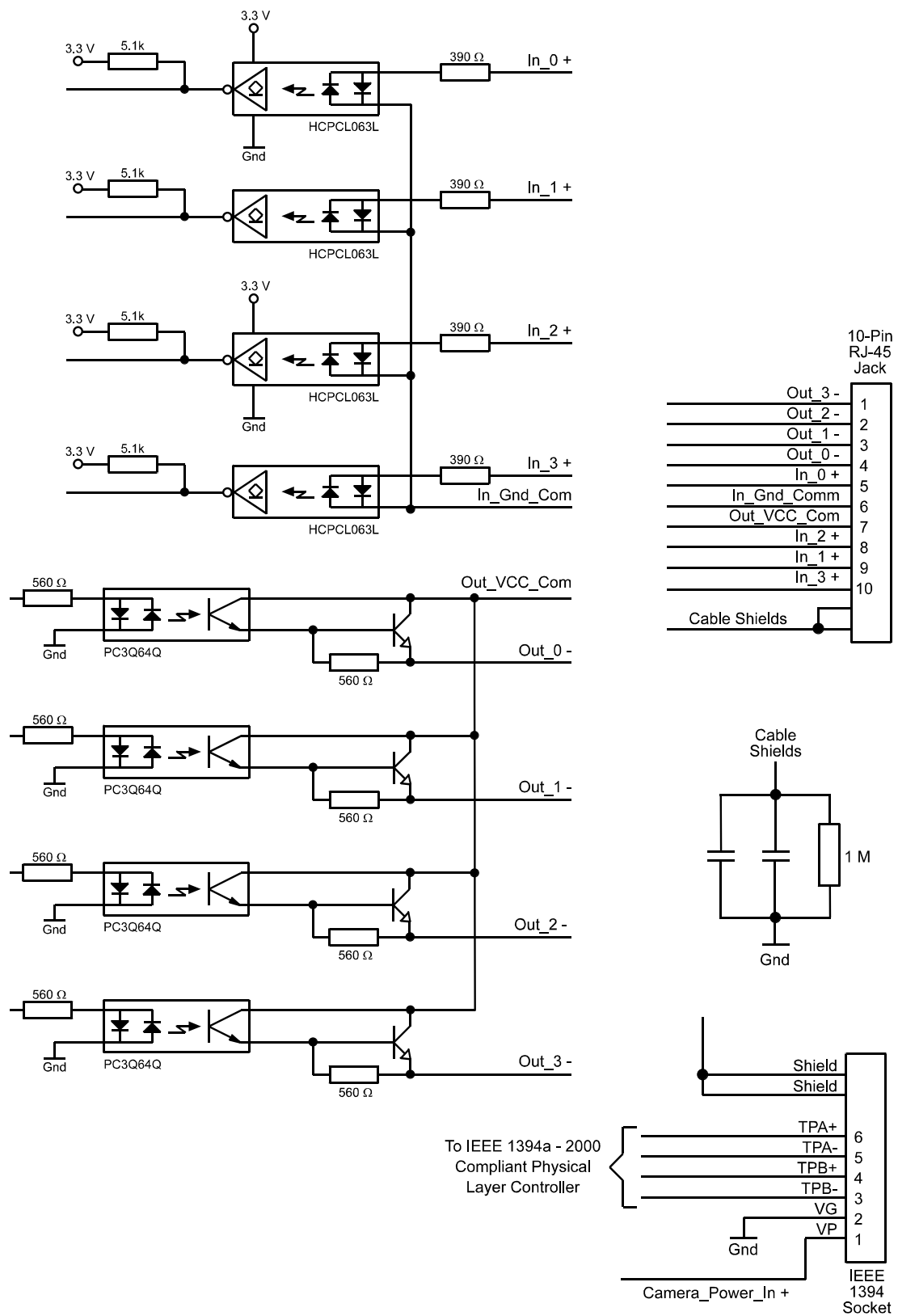
Figure 2-3: I/O Schematic
