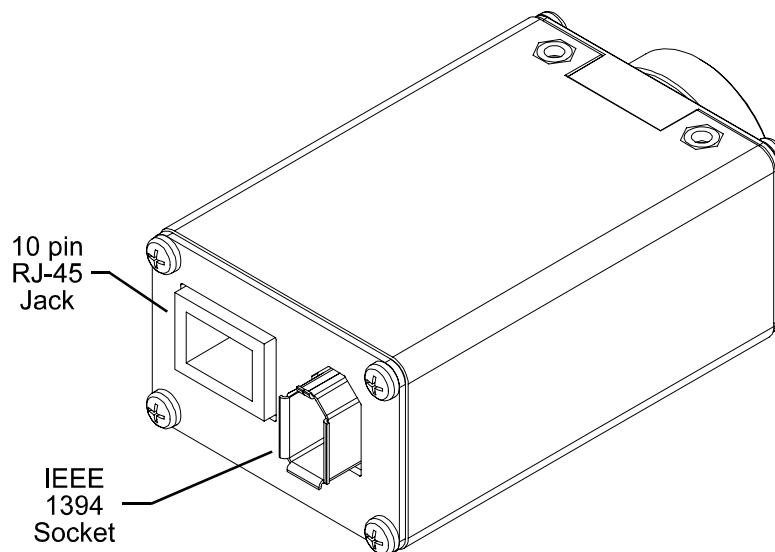
Figure 2-1: Camera Connectors
